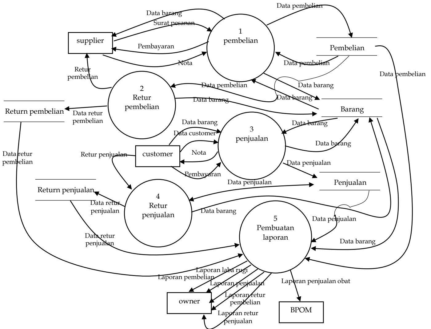
Gambar 6. DFD Level 0
