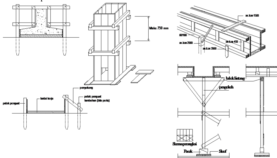
Gambar 1. Macam-macam bekisting
