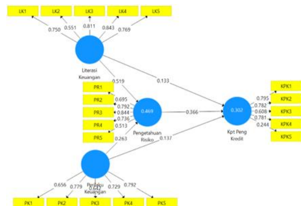
Gambar 1 Output Algorithm
