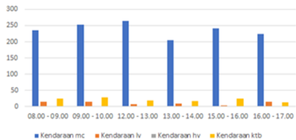
Gambar 6 Volume Lalu Lintas smp/jam
