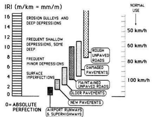
Gambar 3 IRI ( International Roughness Index )
